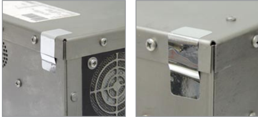
Figure 5.2.1 – Warranty Void stickers Front and Back on the unit
