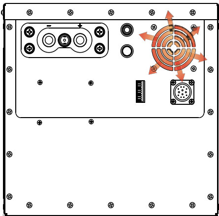
Figure 2.7.2 Front Outlet
