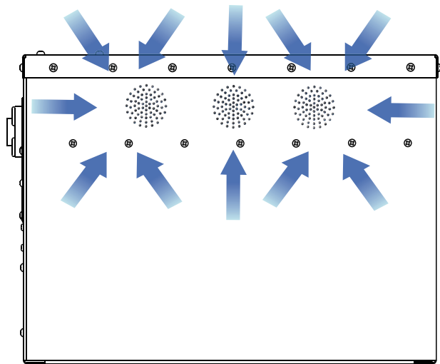
Figure 2.7.3 Back Inlet
