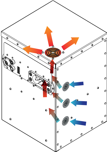
Figure 2.7.1 Airflow
