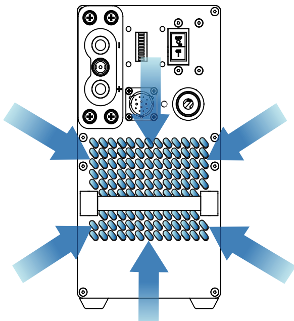
Figure 2.7.3 Front Inlet
