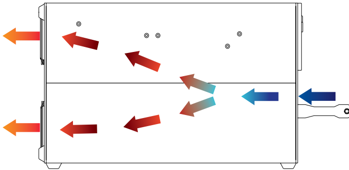
Figure 2.7.1 Horizontal Position
