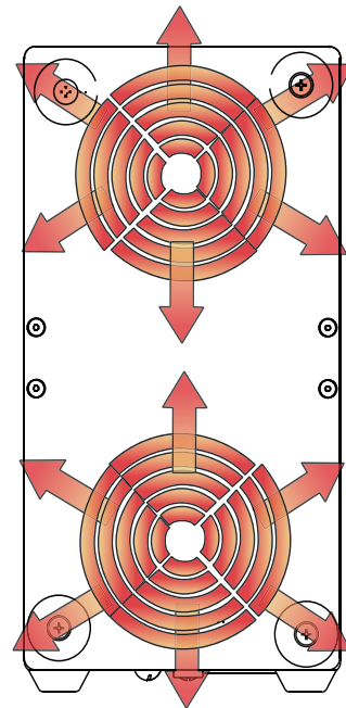
Figure 2.7.4 Rear Outlet
