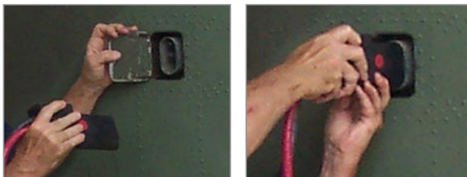
Figure 3.8.3 Attaching DC Power Cable to aircraft
