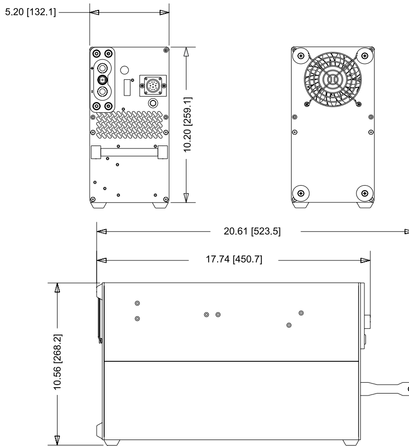
Figure 2.5.1 - TI500 GPU-24 physical dimensions
